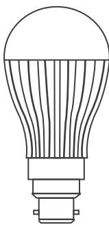
BC Base Diameter: 49.8mm Height: 104mm
