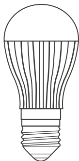
ES Base Diameter: 49.8mm Height: 108mm
